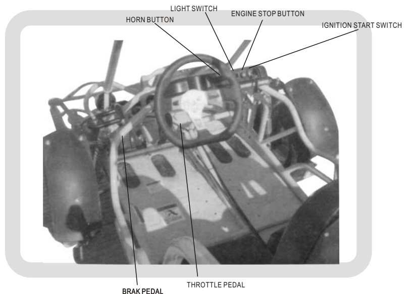
Figure 1 front panel
