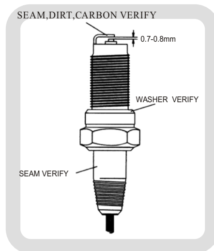
Figure 6 Spark plug
